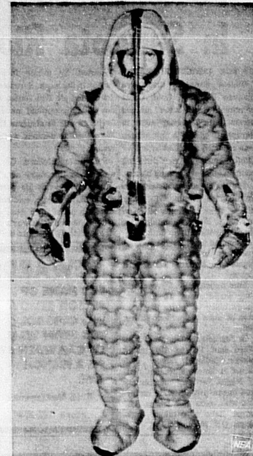
SAFETY SUIT FOR SUBS. The Navy is testing this Mark VII escape suit currently in use by the British submarine service. Once on the surface, the wearer can inflate the suit and float in his own personal "balloon," protected from the elements and in a position of repair.
