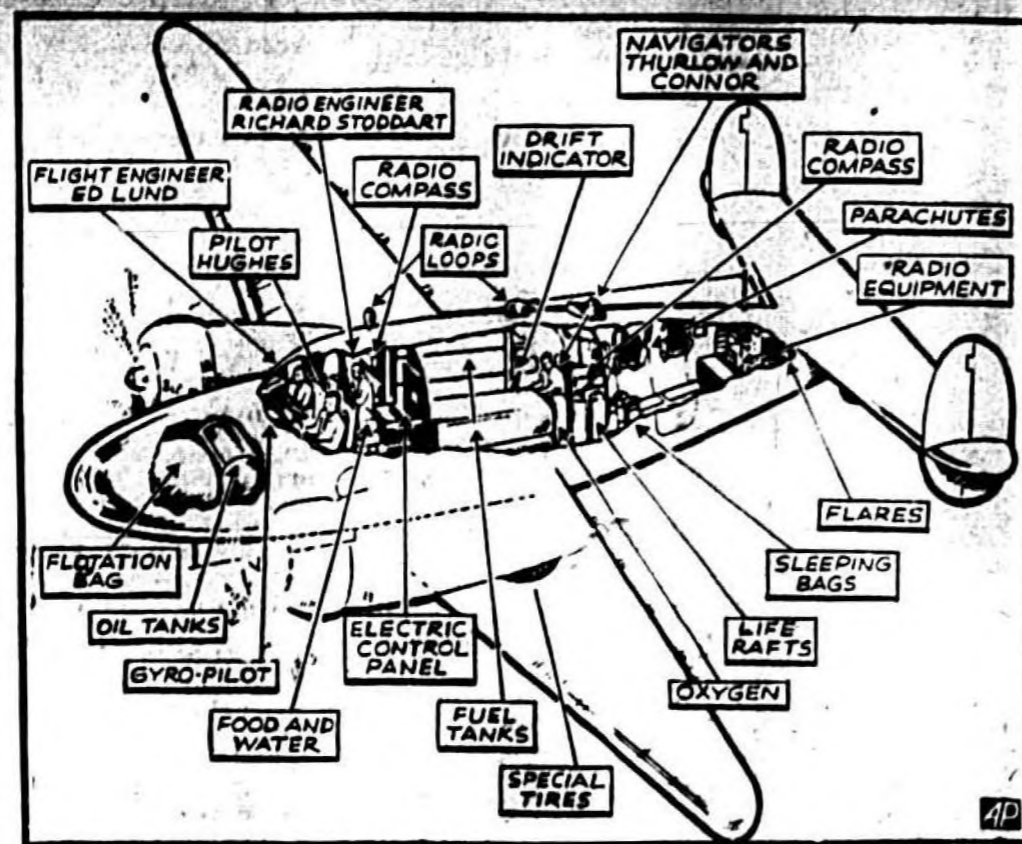
THIS SKETCH indicates how Howard Hughes, his four companions and their equipment are placed in their world-circling plane. They crossed the Atlantic, Europe and Siberia in record-breaking time and headed back to New York via Fairbanks, Alaska.
