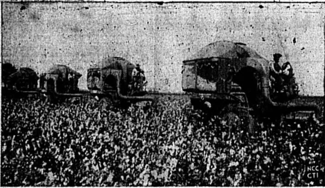
Vanguard of completely mechanized cotton farming, the four giant machines pictured above are typical of the more than 100 mechanical pickers which will aid in harvesting the crop in various sections of the Cotton Belt this fall. The National Cotton Council reports that one of the pickers can harvest more cotton in a few minutes than a hand picker would remove from the field in an entire day. Expanded use of machine pickers will be a big factor in lowering the cost of cotton production.
