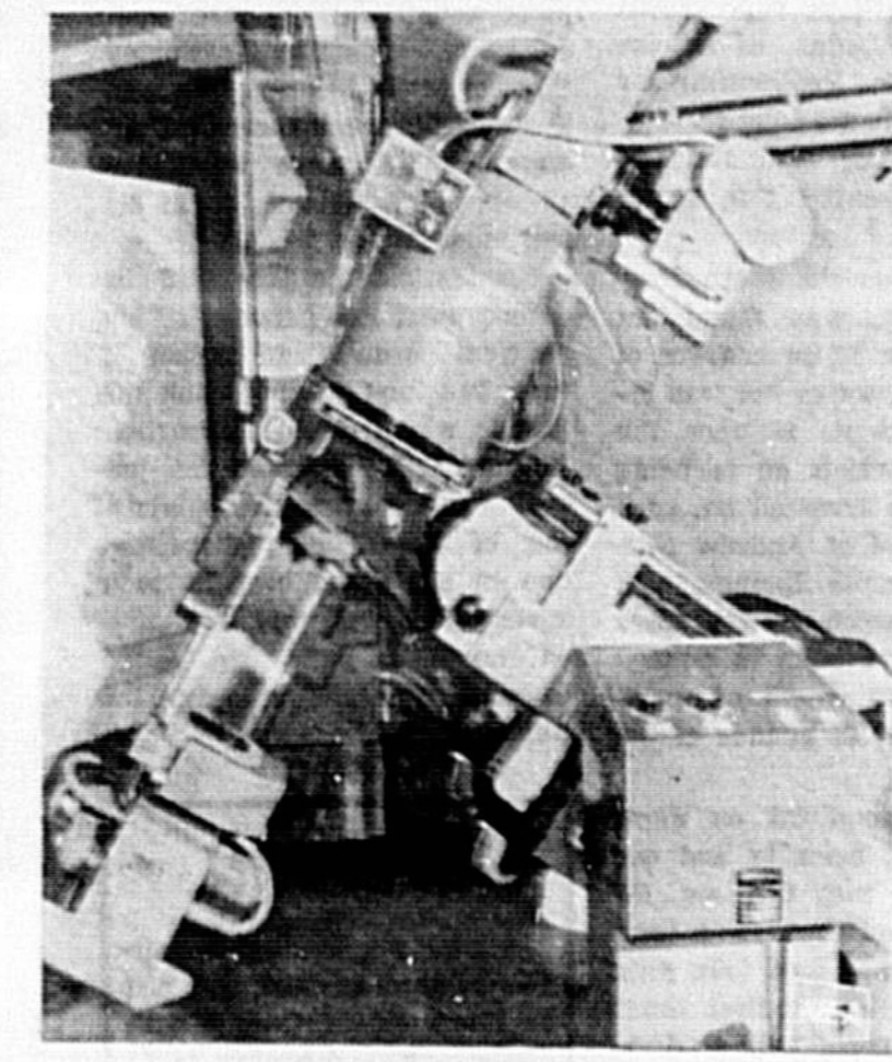
EASY CHAIR? Well, it makes it easy to take X-ray pictures. It's the Plicker chair that rotates a strapped-in patient 360 degrees on a horizontal plane and 230 degrees around the vertical axis to make possible nearly limitless angles for X-ray diagnosis.
