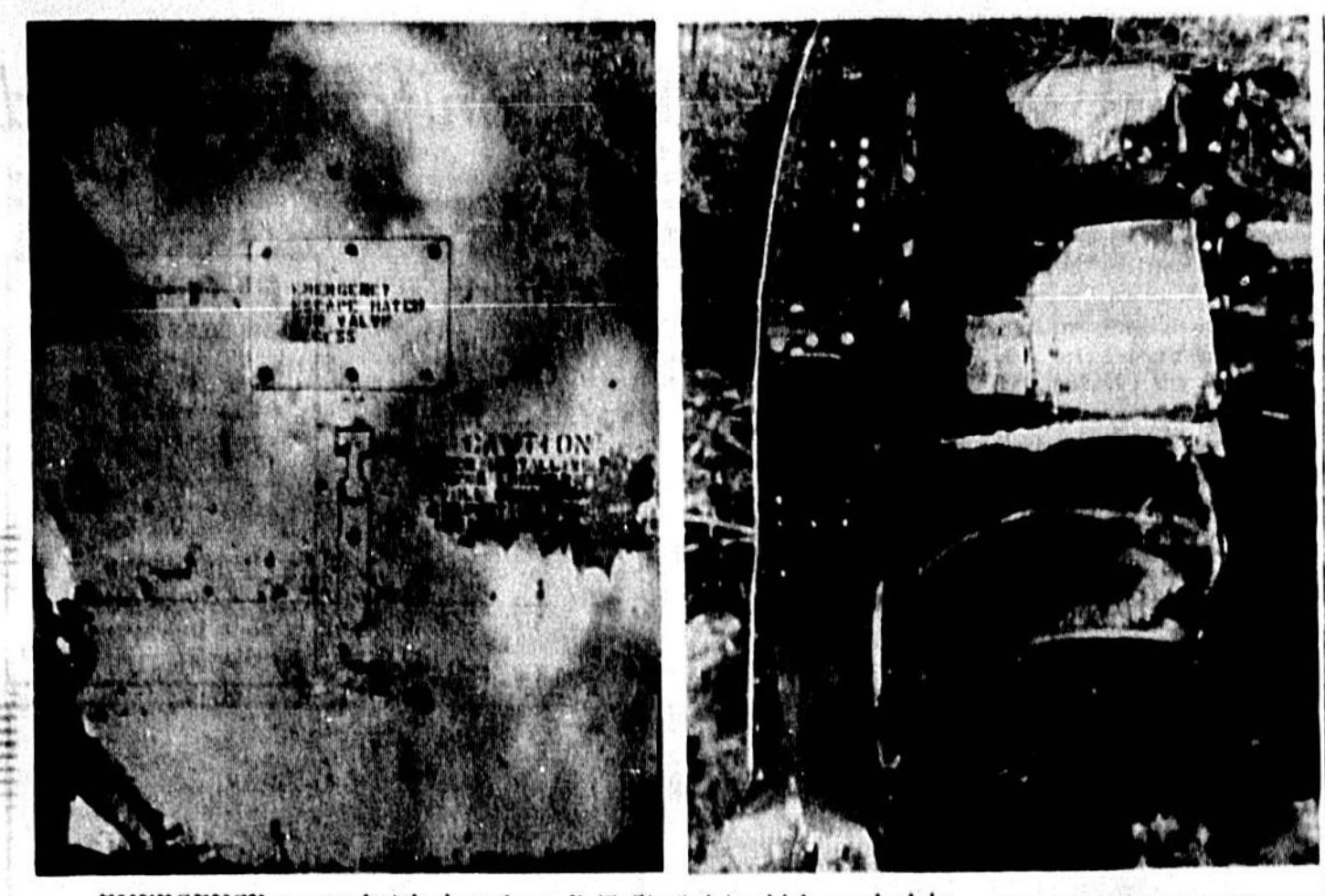
EMERGENCY escape hatch door from B-47 Stratofortress which crashed in 1958 near Chulohota has been unearthed in land clearing operations for new streets in the area. Front view (left) shows lettering to be clearly legible. Door (right) is shown in side position. (Herald Photos)
