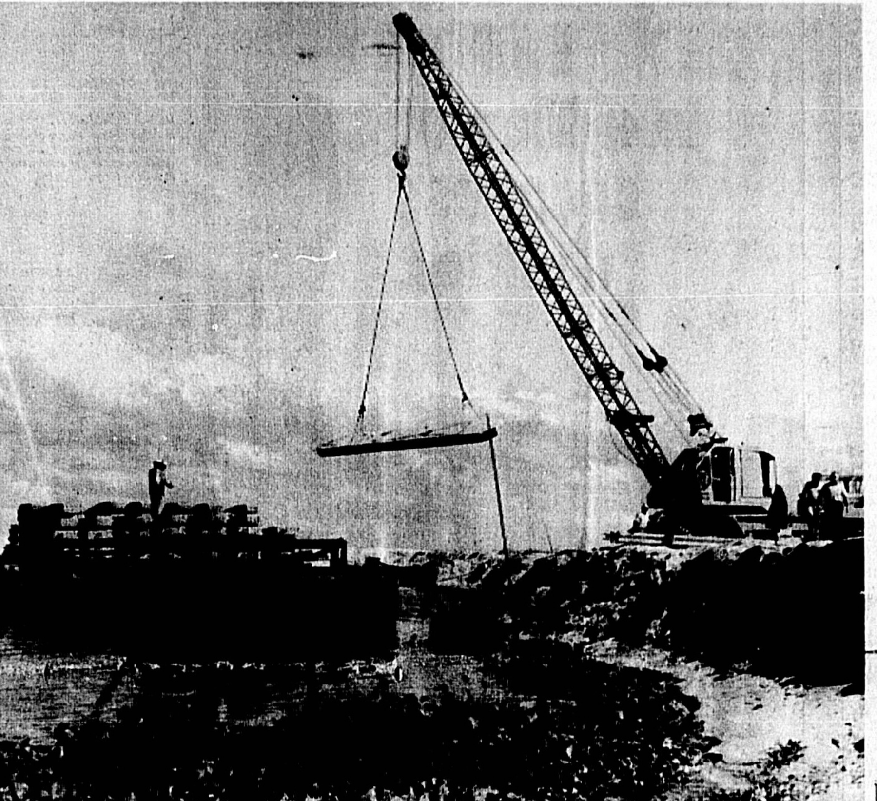
SECOND PHASE of the lakefront development project is underway with unloading on the marina hydraulic fill of concrete bulkhead pilings which will be driven in fill to form walls around the 13-acre land area. Barges loaded with pilings began arriving over the weekend. (Herald Photo)
