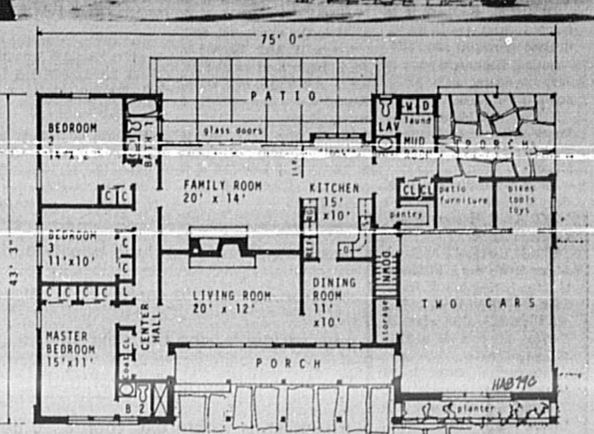
TWIN FIREPLACES in the living and family rooms accent the floor plan of this seven-room ranch plan. There are three bedrooms and two and a half baths in the plan, which contains 1,345 square feet. Use of porches and patios spotlights outdoor living possibilities. Plan HA279C is designed by Lester Cohen, Room 505, 48 W. 88th St., New York, N.Y. 10038. Anyone wishing to know the cost of the blueprint can write to Cohen, enclosing a stamped, self-addressed envelope.
