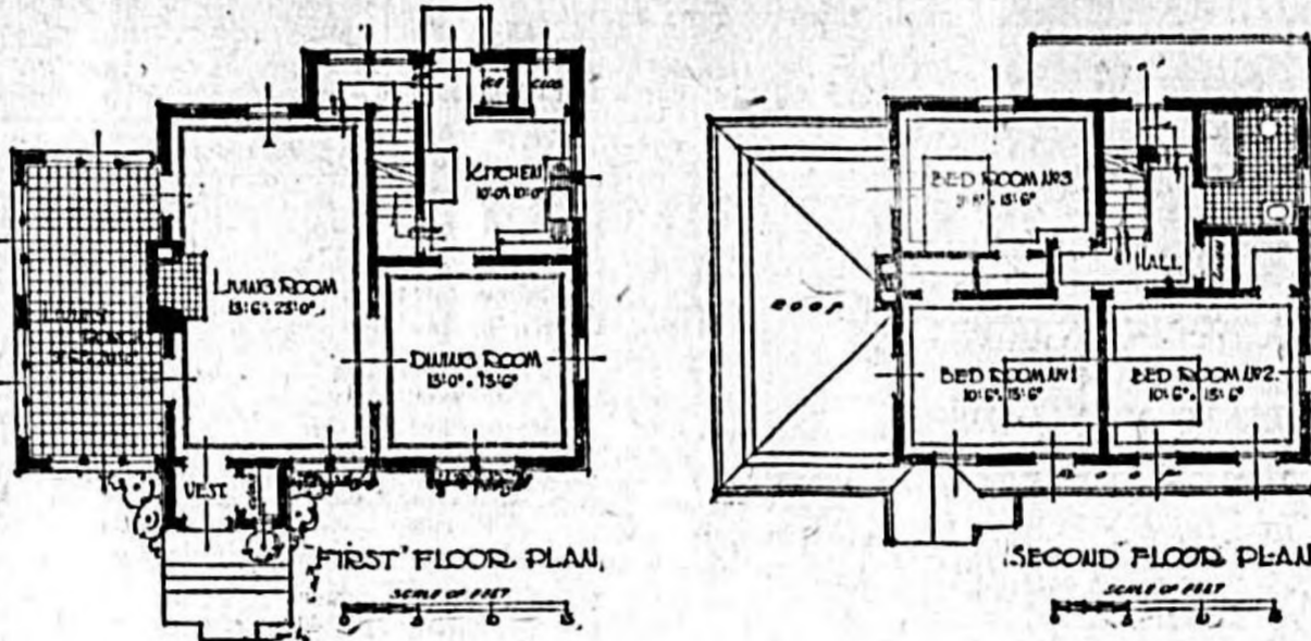
Office of R. C. HUNTER & BRO., Architects. (House A-74.)
