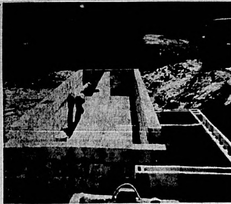
THE FIRST stage of Casselberry Utilities' $12,000 Sewage Treatment Plant expansion program planned in order to accommodate the needs of the Seminole Plaza Shopping Center, is underway. The trickling filter (above) will provide secondary treatment when put into operation and the new chlorine contact chamber (below) will purify the effluent before it flows into the creek. (Herald Photos)
