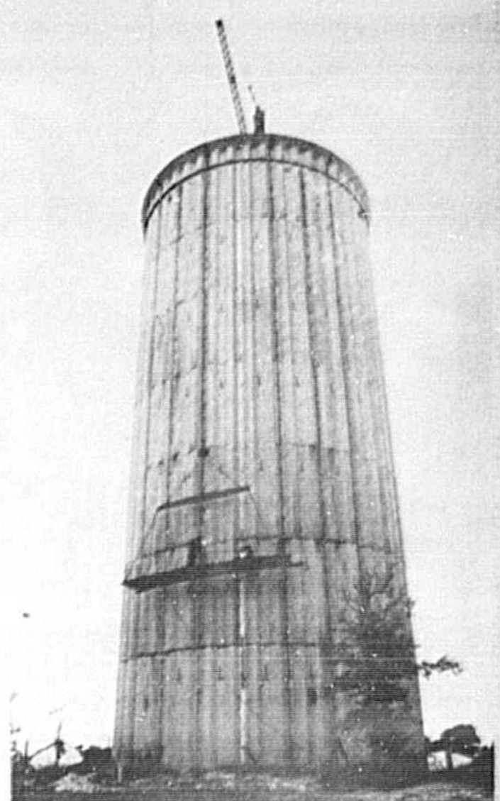
HYDRO PILLAR, a style of water storage tower unique in this area, is being constructed by the City of Altamonte Springs off Palm Springs Road, at the cost of $325,000. The 1 million gallon capacity tank will be mounted on top of this multi-purpose functional silo type base which is 32 feet in diameter at the bottom and will contain office space. The hydro pillar contains 220,000 cubic feet of storage space. (Staff Photos)
