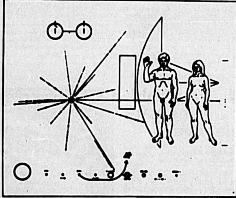
HUMAN MESSAGE carried by Pioneer 10 is inscribed on a 6-by-9-inch metal plate. Nude figures of a man and woman are drawn to scale in front of a recording of the space probe. Other data locate the position of the Earth.
