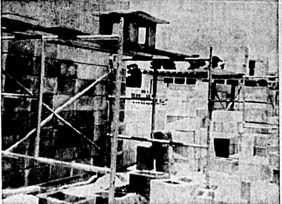
WALLS ARE going up on the new lunchroom at South Seminole Junior High School at Casselberry and work has started on the new band and choral room at the school as well. (Herald Photo)
