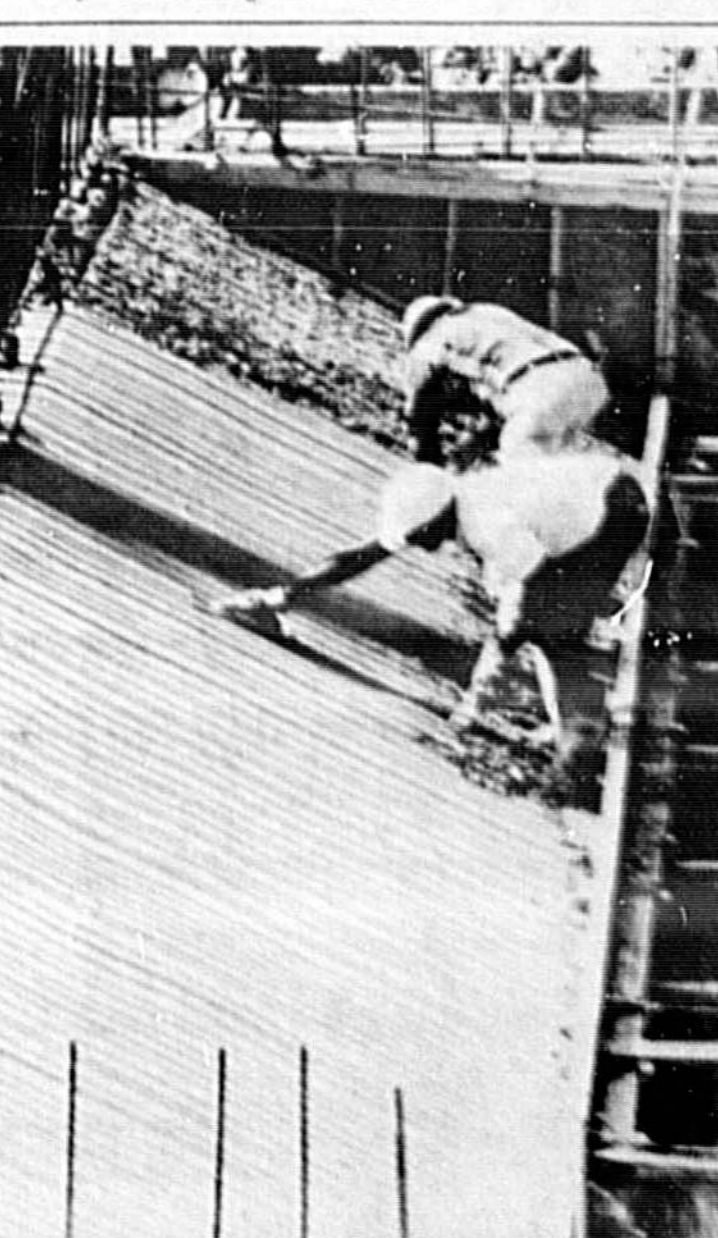
DOWN TO THE NITTY-GRIITY Construction workers have another eight weeks work on a giant grit removal chamber being constructed in $1.3 million expansion of Sanford's lakefront sewage treatment plant. Above, workers trowel concrete on chamber's sloping bottom. More photos on page 1B. (Bob Lloyd Photo)
