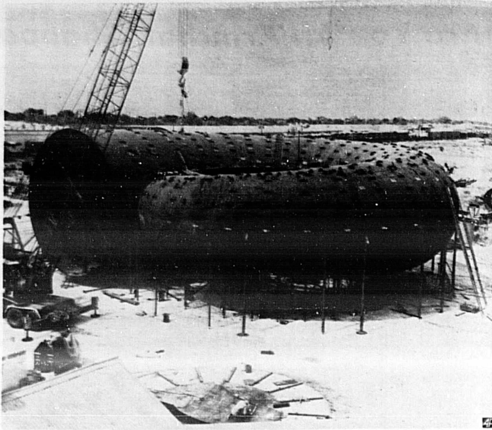
SNAIL OF STEEL — This steel housing, almost 35-feet in diameter at the large end and 7-feet in diameter at the small end, formed in shape of a snail, has been completed in Salt Lake City, Utah. It will be disassembled and shipped for installation in the third powerhouse at Grand Coulee Dam in the state of Washington. The housing was built by a Portland-based contractor.
