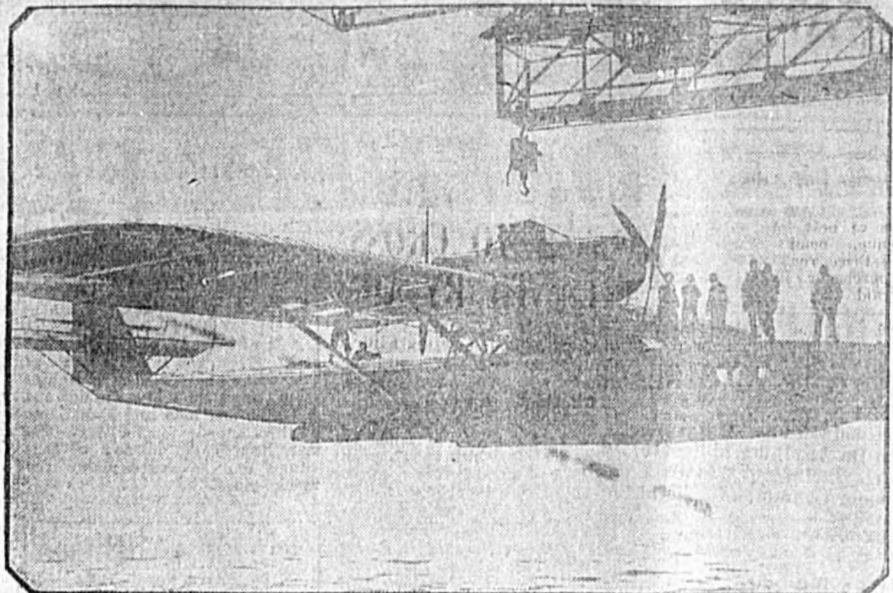
The huge all-metal Dornier "Super-Wal" flying boat, with capacity for 60 passengers, is pictured above. The plane was tested recently at Friedrichshafen, Germany. It is capable of maintaining a speed of 180 kilometers an hour and is equipped with two 500-horsepower Rolls Royce Condor motors in tandem. A plane similar to this will be used by Captain F. T. Courtney, British flyer, in his trans-Atlantic flight, scheduled for the near future.
