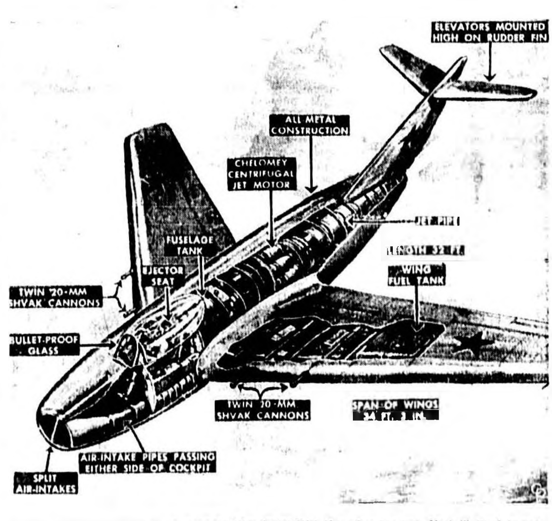
A CASH PRIZE OF $100,000 for information of this Soviet MIG-15 is offered by Capt. Mark W. Clark to any U.S. pilot in North Korea who captures an allied plane. Capt. Clark and his crew were shot down in a MiG-15 on April 22, 1953, and were held in a prison camp in North Korea for 11 months. He was released on May 14, 1953, and returned to the United States.
