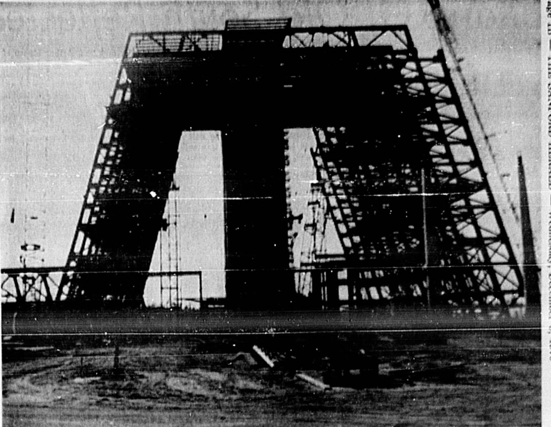
'A' SHAPE begins to rise, as structural steel for Walt Disney World's A-framed Tempo Bay Resort Hotel goes up around the central elevator core for the unique, contemporary-style structure.
