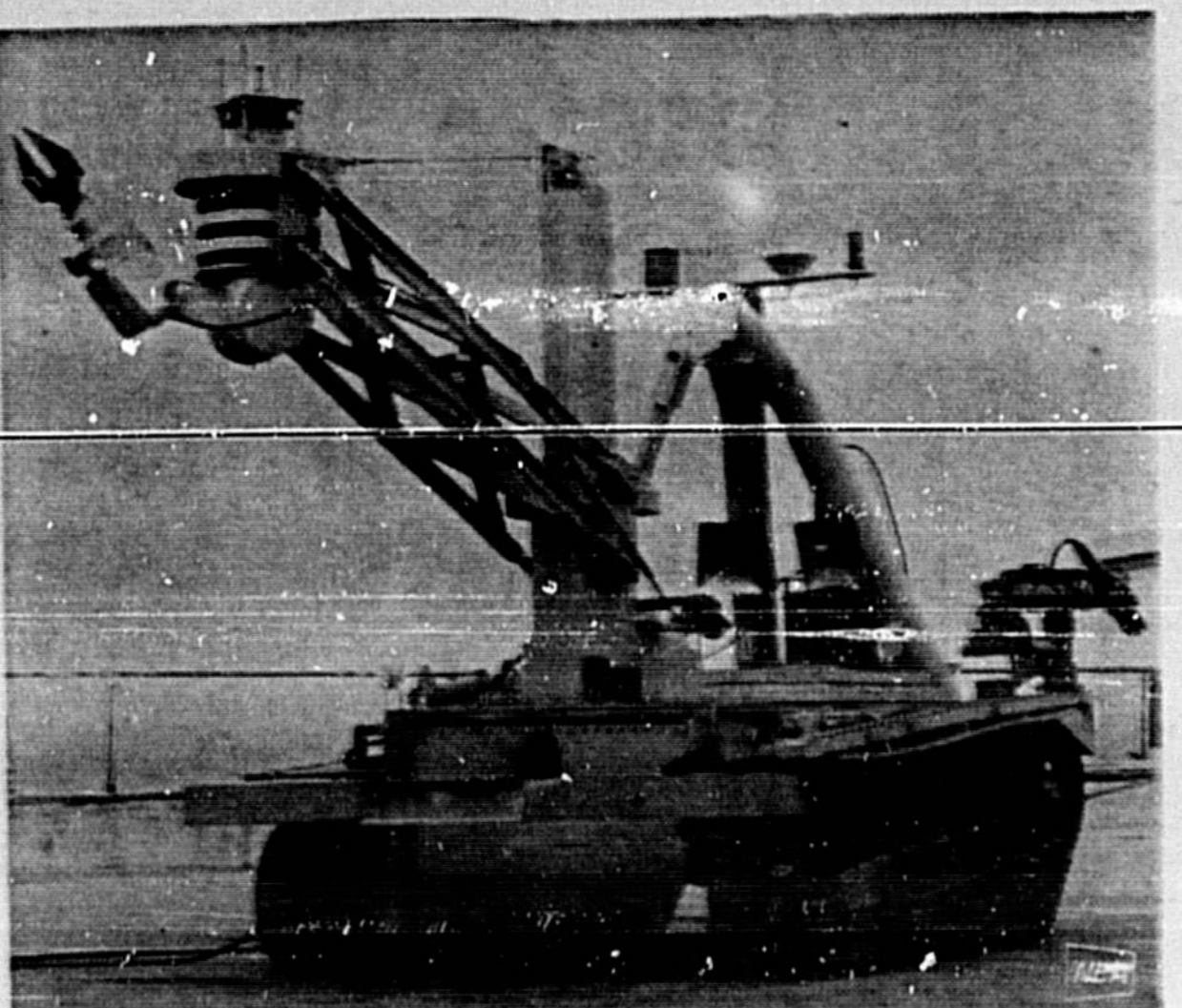
MODERN SEA MONSTER moves, picks up objects and sends pictures from depths of 2,300 feet below ocean's surface. BLM (Hermine Underwater Manipulator) was designed and built by engineers at Scripps Institution of Oceanography in San Diego, Calif. It currently is making tracks along the sea bottom in offshore trials near La Jolla.
