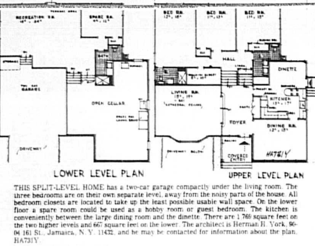
THIS SPLIT-LEVEL HOME has a two-car garage compactly under the living room. The three bedrooms are on their own separate level...
