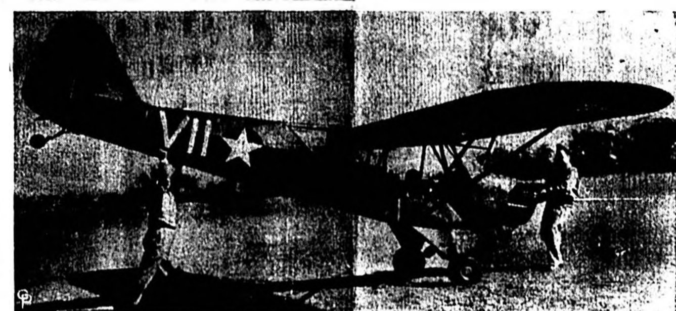
OBSERVATION BALLOONS for directing artillery fire are outmoded. In their place, the U. S. Army is using light, inexpensive planes like this one for a flight somewhere in England. It is called a "flying jeep" by the Army.
