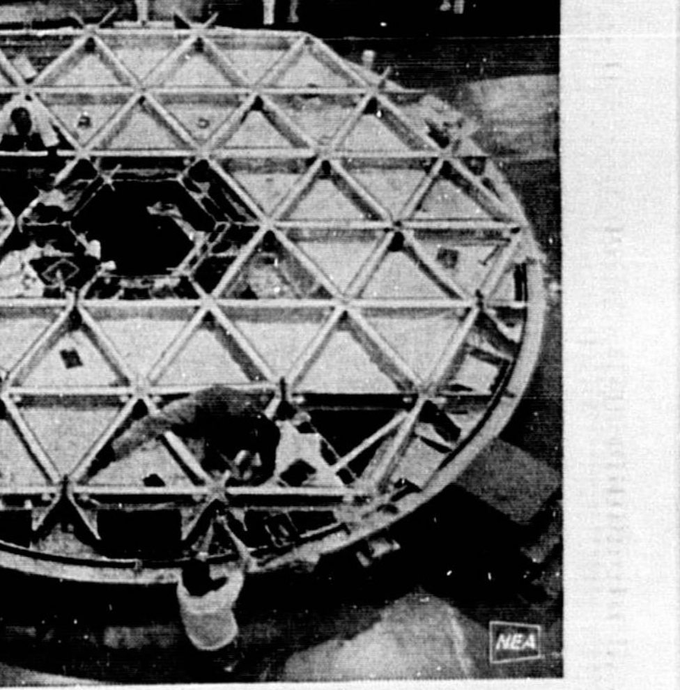
LIKE BEES in a honeycomb, technicians swarm over 22-foot diameter floor for Skylab's Saturn Workbox. This is one of two floors in the embryonic space station being readied for launch in 1972. Workman in a Saturn upper stage and will have 10,000 cubic-foot area in which a three-man Apollo crew will live and work.
