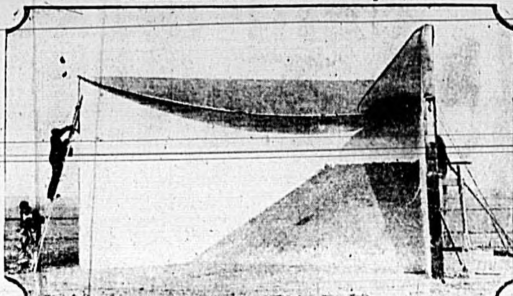
SNAPPED AT ROOSEVELT FIELD, L. I.—A view of the perfected Adams air mail pick-up, which has been successfully tested by pilots dropping mail bags into it and picking up other bags from it and which now will be used as a refueling station for a plane in flight. The Travelair monoplane Postmaster General, piloted by Capt. John O. Donaldson, L. V. Rawlings and Leon Brown, will go up with a light load and refuel as they fly in an attempt to break the world's endurance record.
